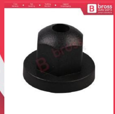
BCF1852 10 Pieces Screw Nut for VW Audi Head Diameter 14.1 mm Stem Diameter 8.9mm
