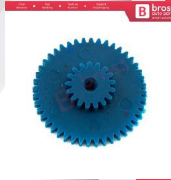
BGE653 VDO Speedometer Odometer Kilometer Cluster Repair Gear Cog 44x17 Teeth
