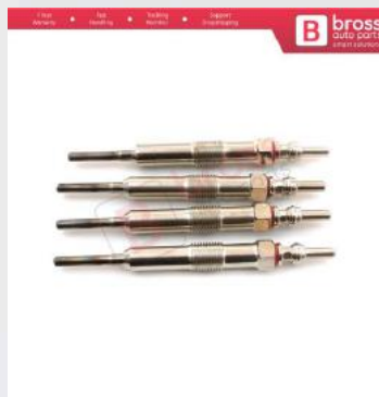
BGP104-1 4 Pieces Glow Plug Auxiliary Heater 4.4 Volt 8200682592 for Renault Dacia Mercedes Nissan 1.5 dCi Engine
