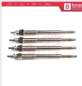
BGP60-1 4 Pcs Heater Glow Plugs GJ1135KI 0100226522 for Kia Hyundai 1.1 1.4 1.6 CRDI
