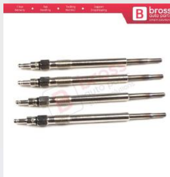
BGP5-1 4 Pcs Heater Glow Plugs N10579805 MN980406 GX3117 0106671802 for VW Audi Seat Skoda Mitsubishi
