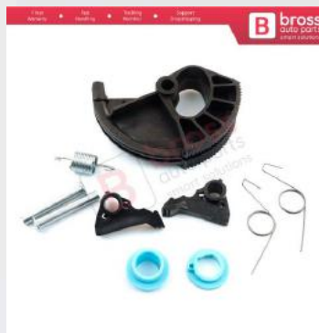
BSP598 Clutch Controls Adjuster Quadrant Pawl Kit for Renault Clio Symbol
