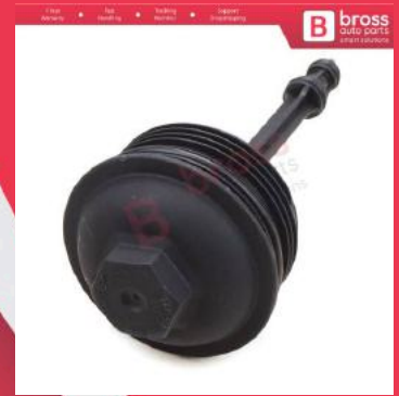
BSP767 Oil Filter Cap 03L115433 for VW Audi Seat Skoda 1.6 2.0 Diesel
