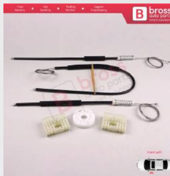
BWR5170 Window Regulator Repair Kit Front Left for Audi A2 8Z 8Z0 1999-2005 5-Door Hatchback 8Z0837461
