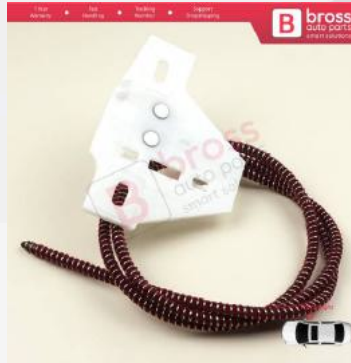
BWR5175 Monorail Window Regulator Repair Kit Right Door for Renault Master MK2 Mascott Opel Movano A Iveco Daily 3 4 Nissan Interstar X70
