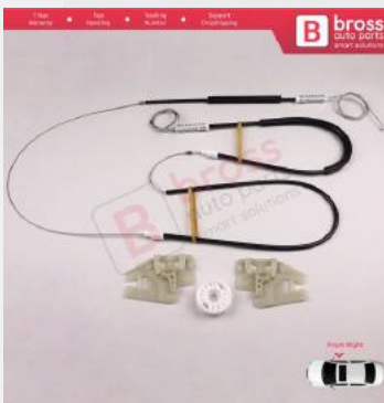
BWR492 Window Regulator Repair Kit Front Right Door for BMW 3 Series E46 2001-2005 4/5 Door Facelift 51337020660
