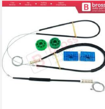
BWR231 Window Regulator Repair Kit Front Left Door for Audi A6 C5 4B 1997-2005 Allroad 4BH 4/5 Door 4B0837461
