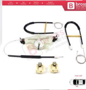
BWR421 Power Window Regulator Repair Set Front Left Door for Seat Leon MK1 1M1 1999- 2006 Seat Toledo MK2 1M2 1998-2004 4/5 Door 1M0837461A
