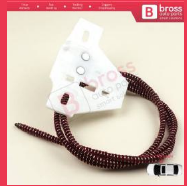
BWR5175 Monorail Window Regulator Repair Kit Right Door for Renault Master MK2 Mascott Opel Movano A Iveco Daily 3 4 Nissan Interstar X70
