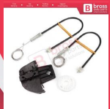
BWR5510 Power Window Regulator Repair Kit Rear Left Door for VW Touran MK1 1T1 1T2 1T3 2003-2015 1T0839461
