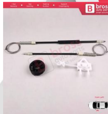
BWR5295 Power Window Regulator Repair Set Front Left for Fiat Albea Siena Palio MK1 171 172 178 1996-2016 4/5 Door 46786201
