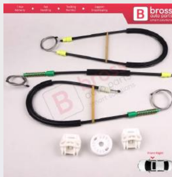
BWR633 Window Regulator Repair Set Front Right Door for Peugeot 607 9D 9U 1999-2010 9222Q0
