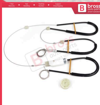
BWR5519 Power Window Regulator Repair Kit Front Right Door for VW CC Passat CC 357 358 2008-2017 4-Door Comfort Coupe Sedan 3C8837462
