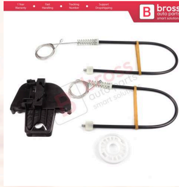
BWR5511 Power Window Regulator Repair Kit Rear Right Door for VW Touran MK1 1T1 1T2 1T3 2003-2015 1T0839462
